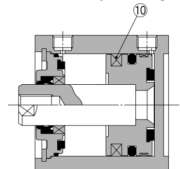
With auto switch (Built-in magnet)
