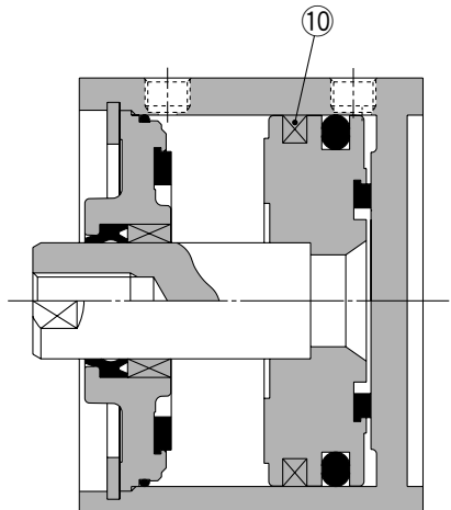
With auto switch (Built-in magnet)
