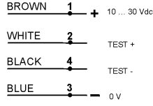
S5-5-G8/G12 (4 wires)
