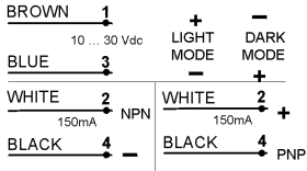
S5-5-x (4 wires)
